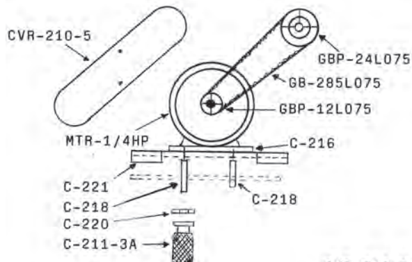
BRUSH DRIVE MODEL 5, 10, 20
