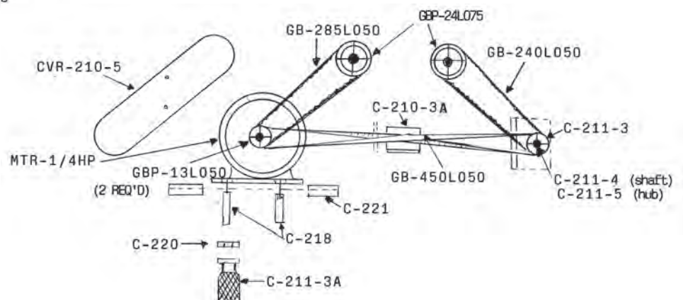
BRUSH DRIVE MODEL 5 BUILT PRIOR 2000
